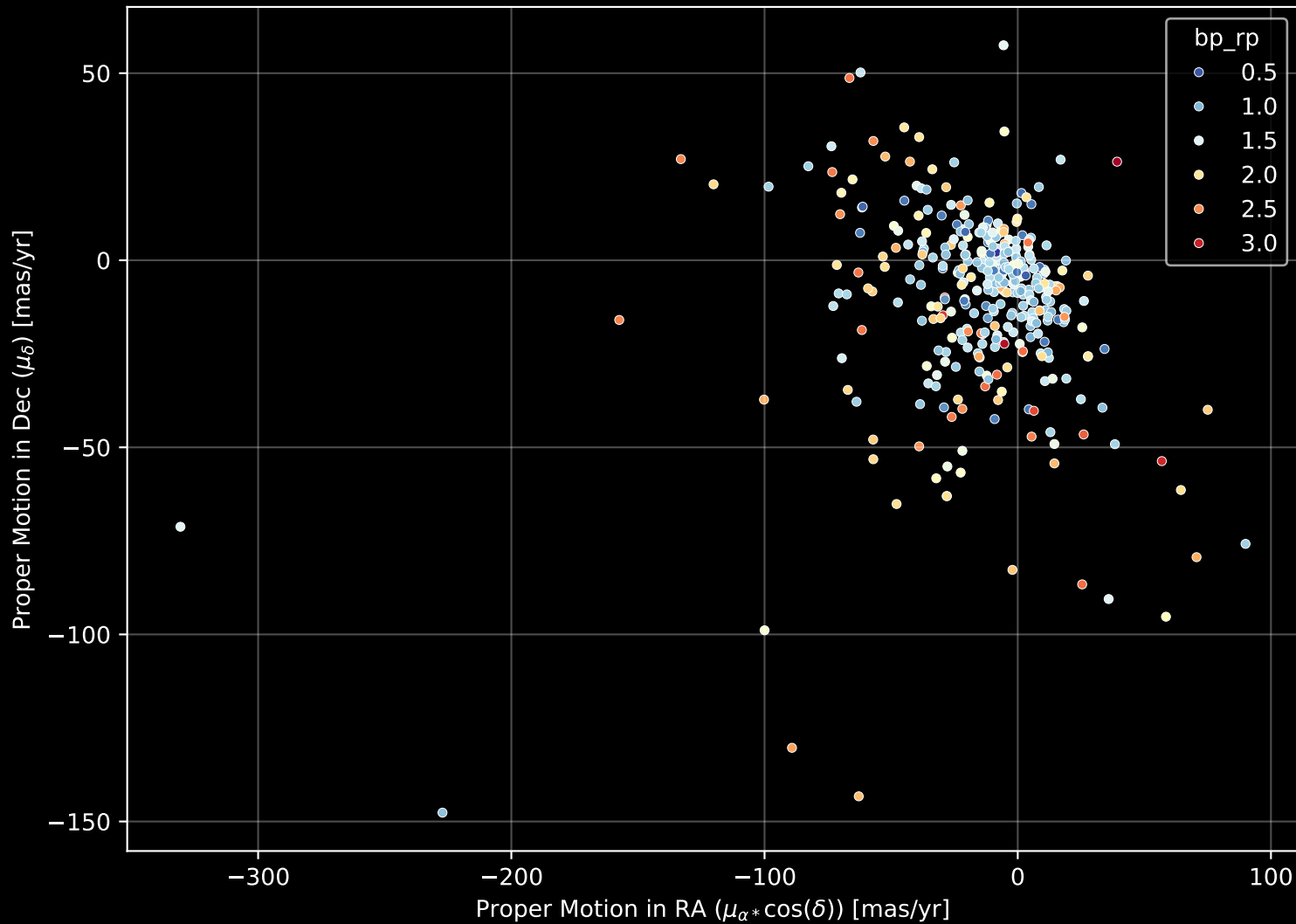
APOGEE DR17 Field: [090+75] Proper Motion Diagram (n= 366)
