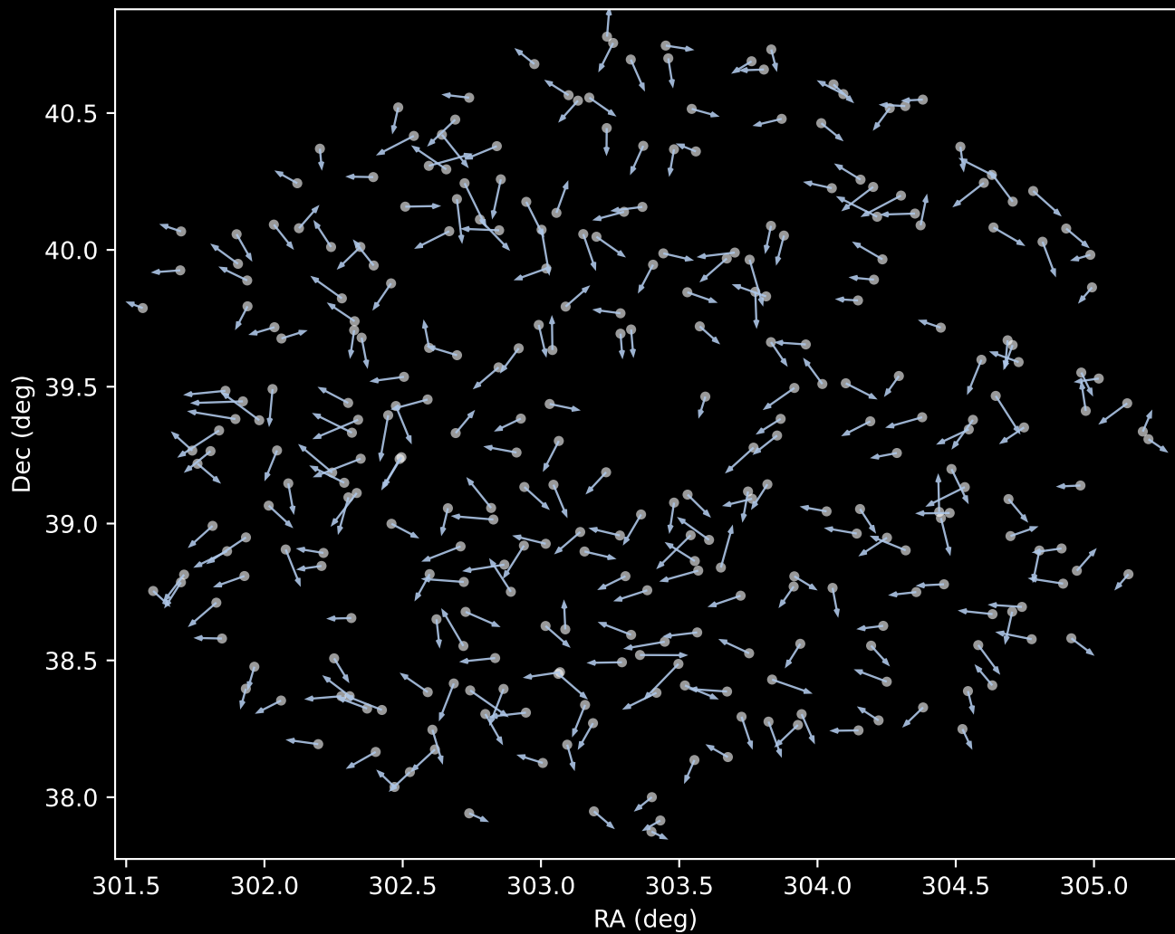
APOGEE DR17 Cluster 1 Proper Motion Vectors (n=306)
