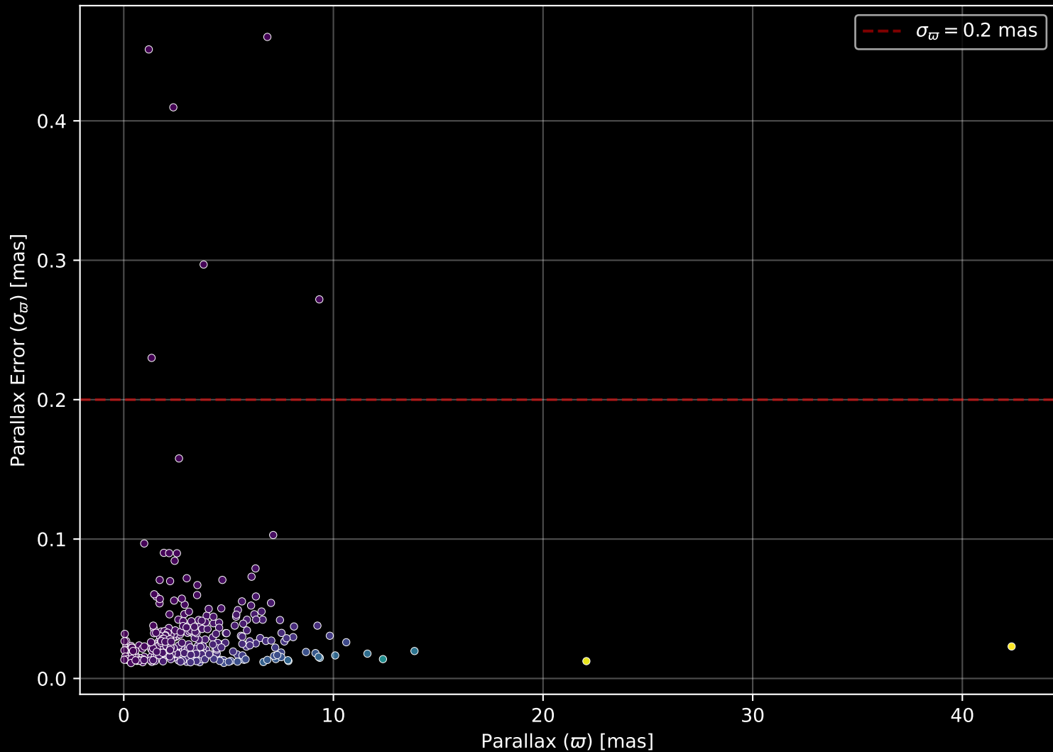
APOGEE DR17 Field: [090+75] Parallax Quality (n= 366)
