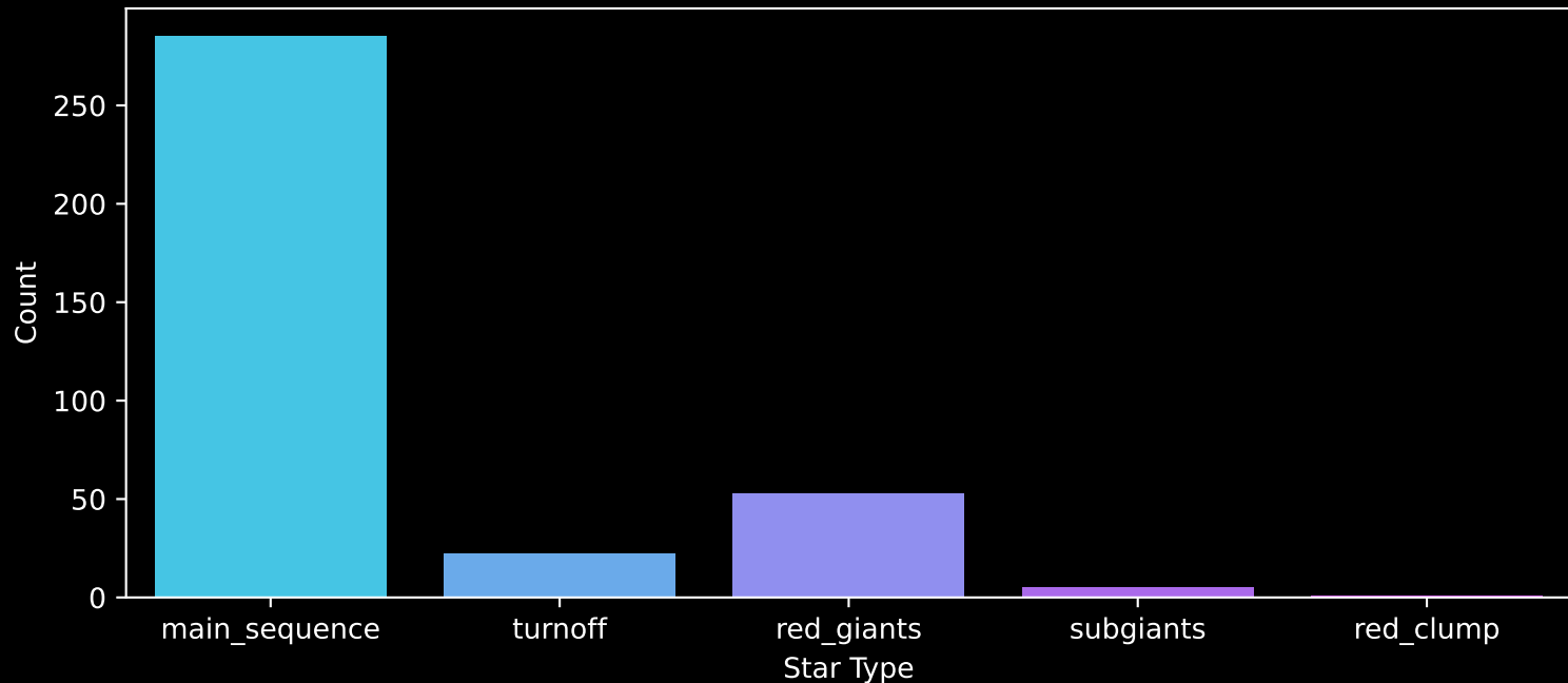
APOGEE DR17 Field: [090+75] Count plot of Star Type
