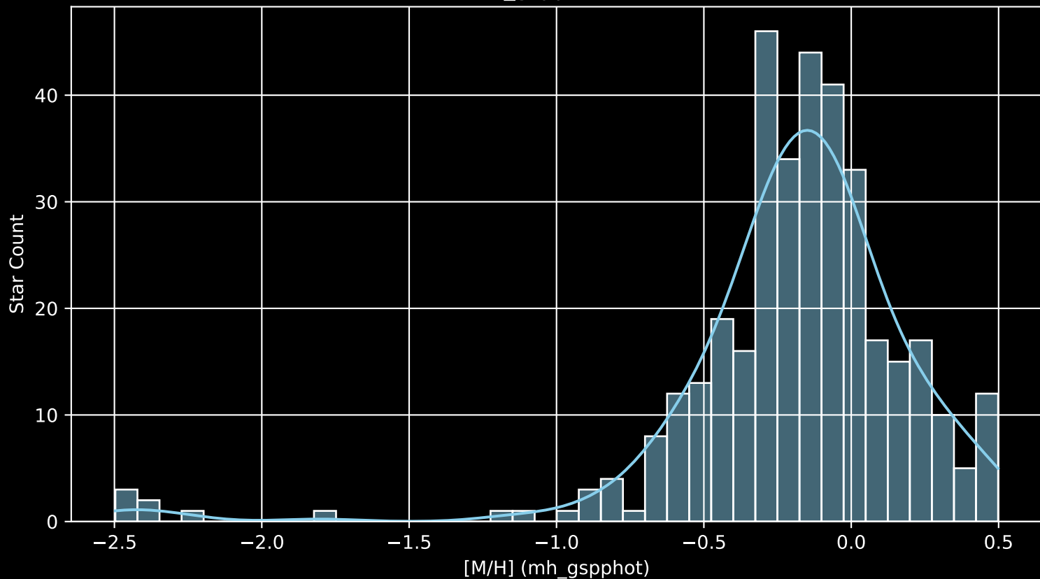
APOGEE DR17 Field: [090+75 [M/H] (mh_gspphot) (n= 360)
