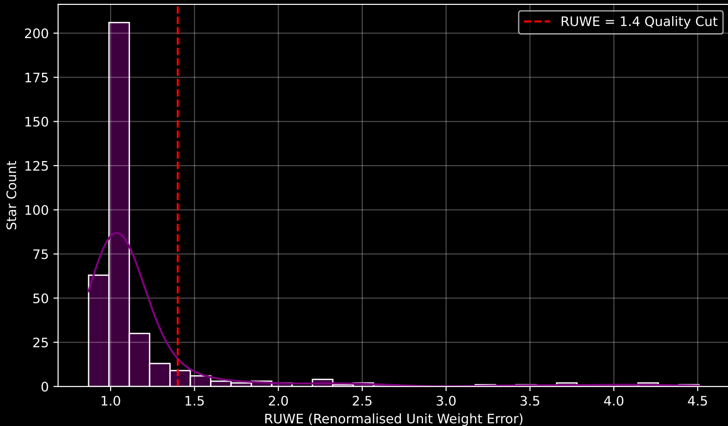
GAPOGEE DR17 Field [090+75] RUWE Distribution (n= 354)
